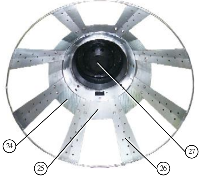
40" & 42" Fan heater burner assembly.
